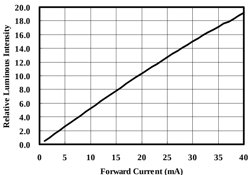
Relative Luminous Intensity vs. Forward Current (Ta=25°C)
